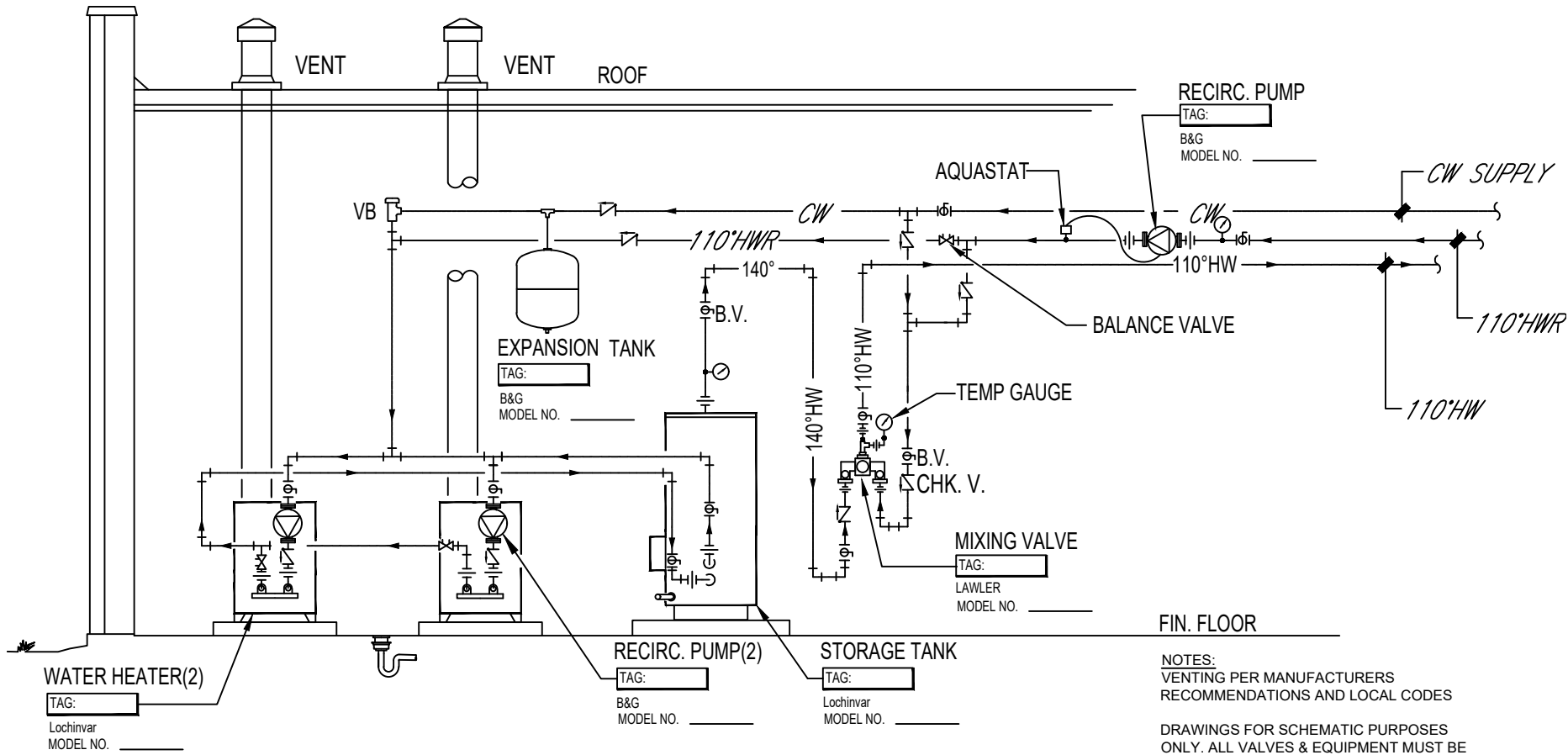
TWO CONDENSING HEATERS, ONE TANK, SINGLE TEMPERATURE
